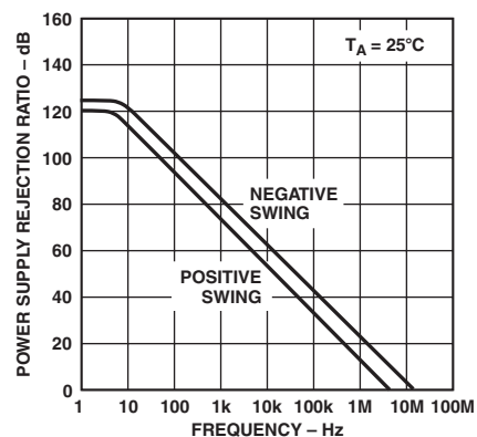
TPC 31. PSRP vs. Frequency
