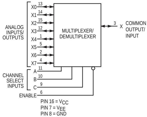
LOGIC DIAGRAM MC74VHC4051 Single-Pole, 8-Position Plus Common Off
