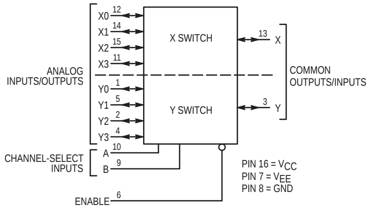
LOGIC DIAGRAM MC74VHC4052 Double-Pole, 4-Position Plus Common Off
