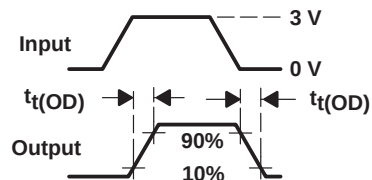
VOLTAGE WAVEFORMS
