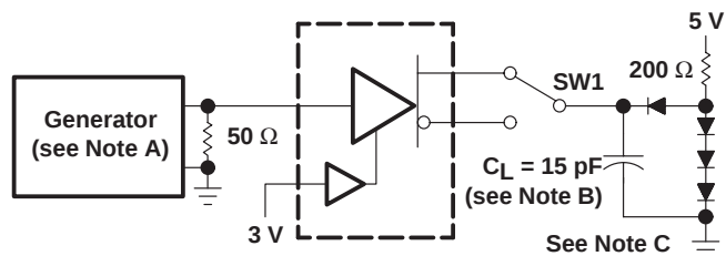
TEST CIRCUIT
