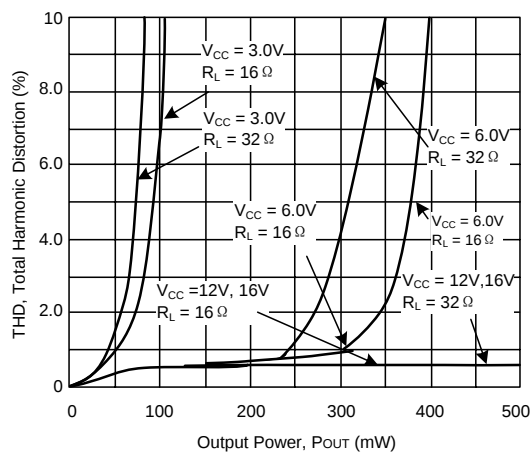
Distortion Versus Power ( f = 1.0\text{kHz} , \text{AVD} = 34\text{dB} )
