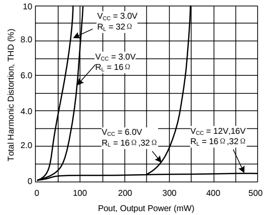
Distortion Versus Power ( f = 1, 3.0\text{kHz} , \text{AVD} = 12\text{dB} )
