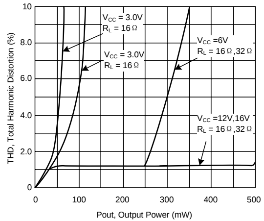
Distortion Versus Power ( f = 3.0\text{kHz} , \text{AVD} = 34\text{dB} )
