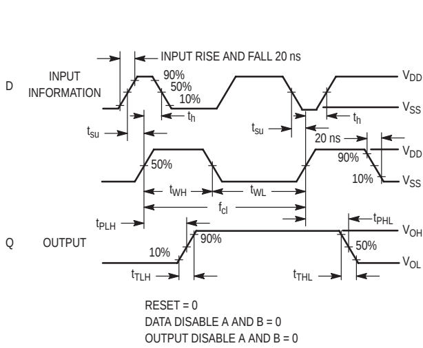
Figure 1. Timing Diagram
