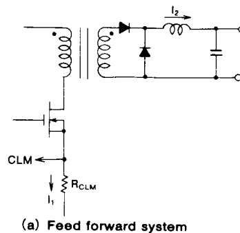
(a) Feed forward system
