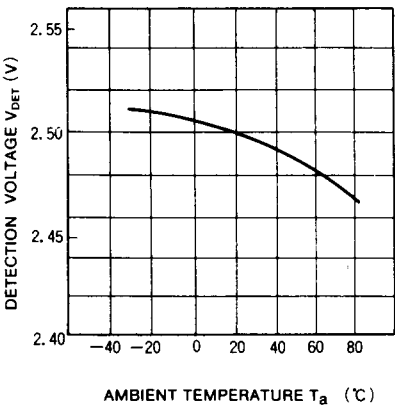
DETECTION VOLTAGE VS. AMBIENT TEMPERATURE
