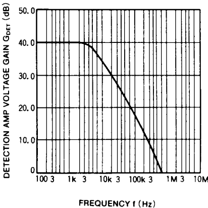
DETECTION AMP VOLTAGE GAIN VS. FREQUENCY
