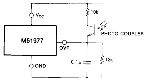
Fig. 28 Peripheral circuit of OVP terminal
