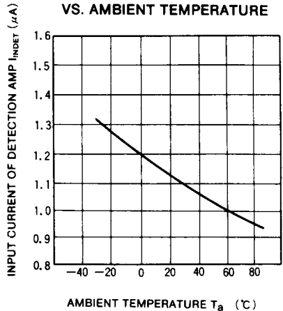
INPUT CURRENT OF DETECTION AMP VS. AMBIENT TEMPERATURE
