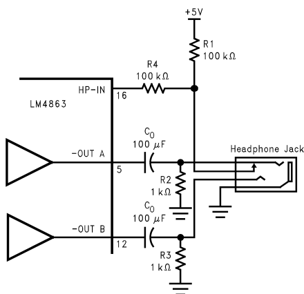
FIGURE 2. Headphone Circuit
