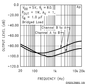
Channel Separation
