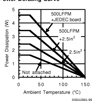
LM4863MTE (Note 16) Power Derating Curve
