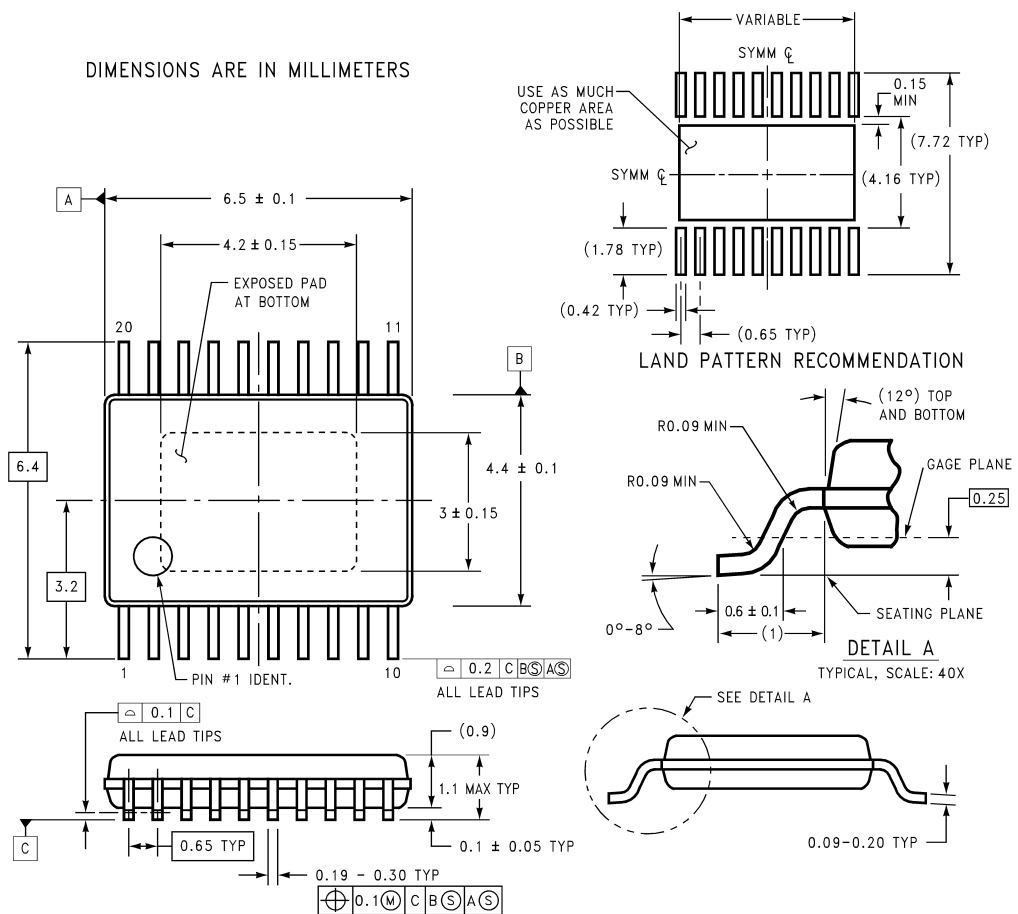
20-Lead Molded TSSOP, Exposed Pad, 6.5x4.4x0.9mm Order Number LM4863MTE NS Package Number MXA20A
