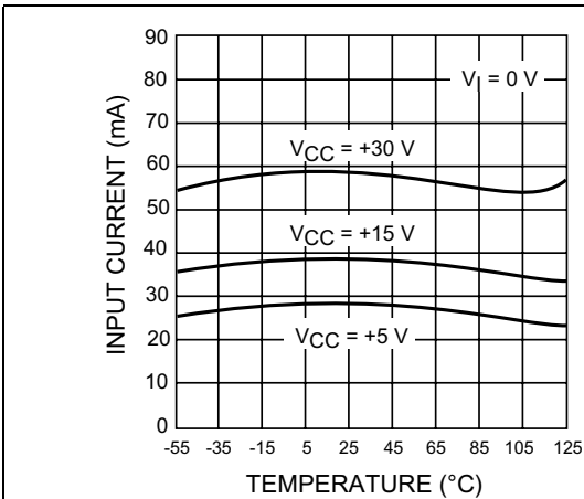
Figure 6. Input current
