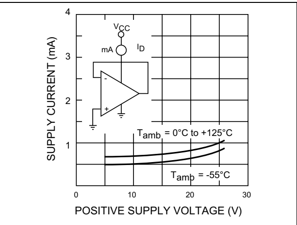
Figure 13. Supply current
