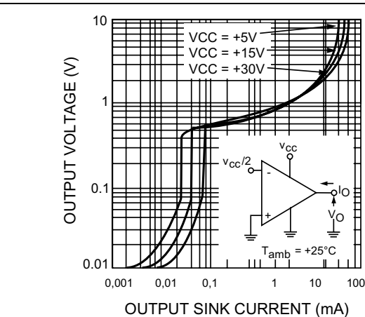
Figure 7. Output characteristics
