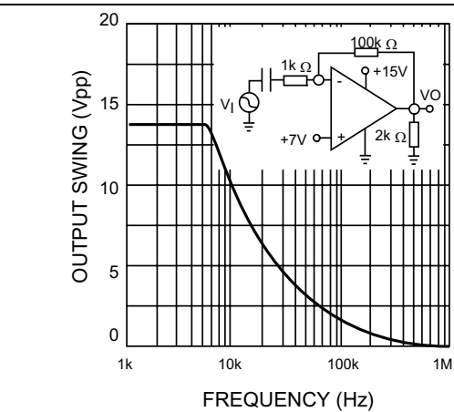
Figure 3. Large signal frequency response
