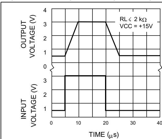
Figure 4. Voltage follower pulse response
