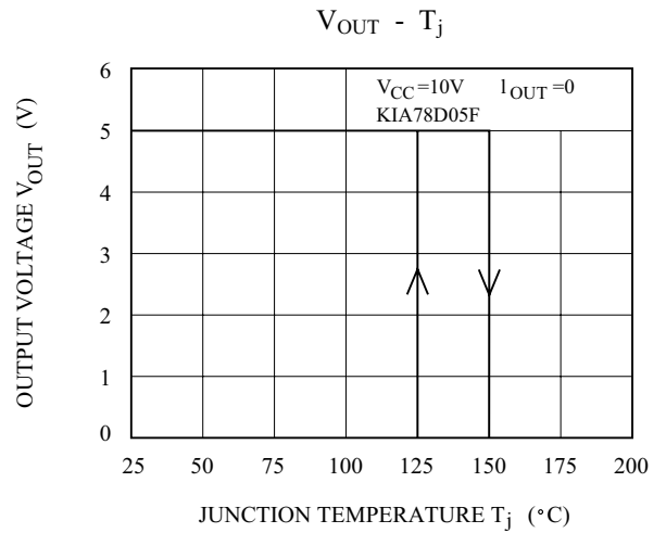
Fig 4. Thermal CATT Circuit Characteristics.
