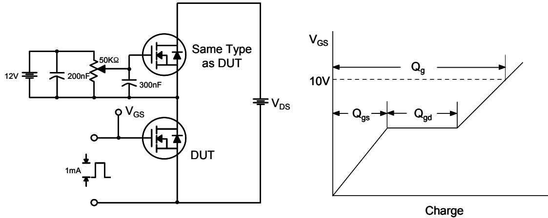
Fig. 13. Switching Time Test Circuit &amp; Waveforms
