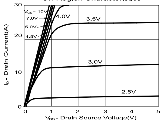
On-Region Characteristics
