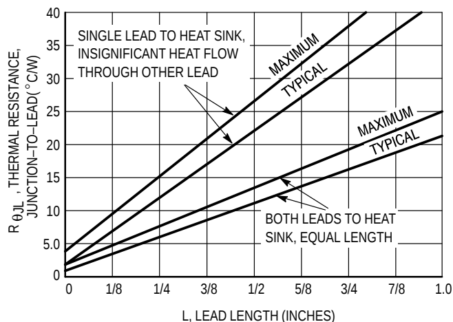
Figure 8. Steady State Thermal Resistance
