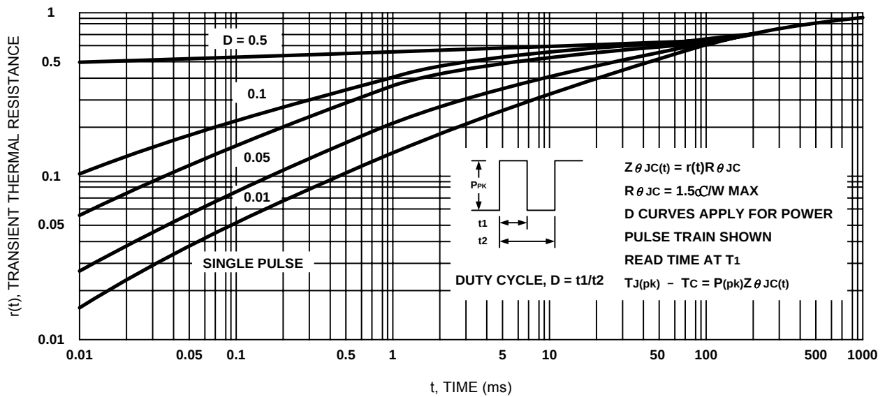
Figure 6. Thermal Response
