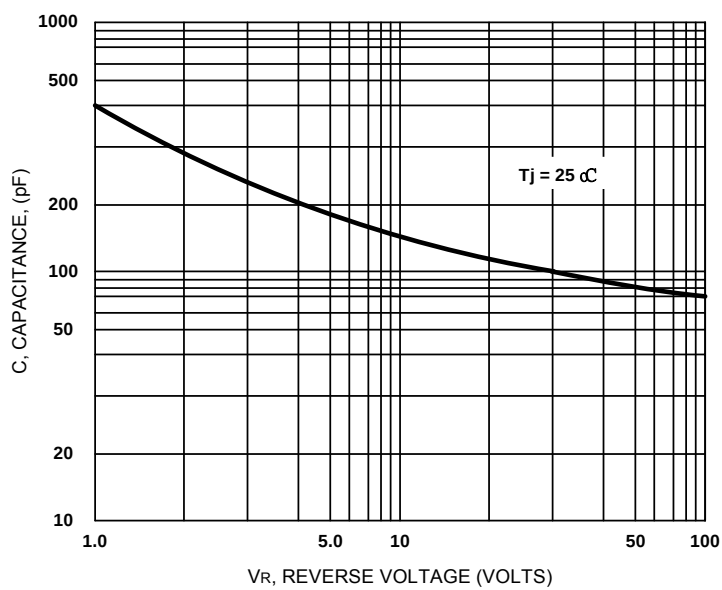
Figure 7. Typical Capacitance
