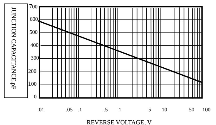
FIG.4-TYPICAL JUNCTION CAPACITANCE
