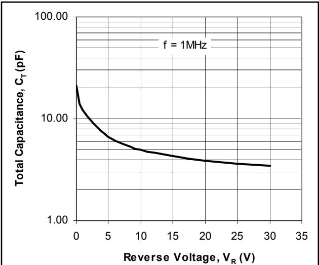
Fig. 3. Typical Capacitance
