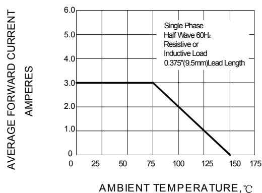
FIG.3 -- FORWARD DERATING CURVE
