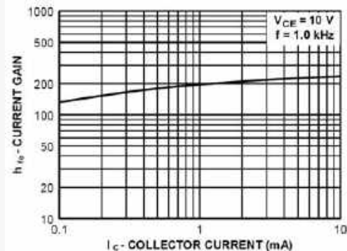
Figure 15. Current Gain
